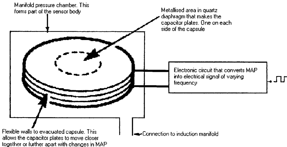
Fig. 5.23 Principle of a capacitive-type MAP sensor
