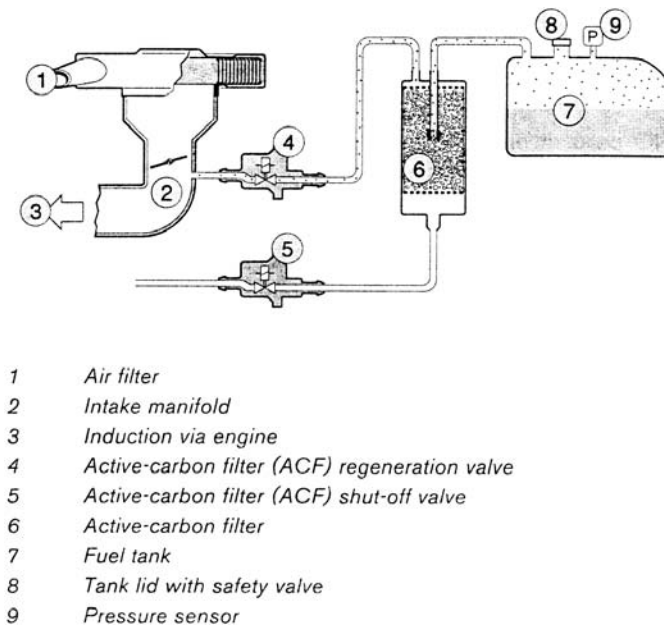
Fig. 8.16 The elements of a leakage detection system
