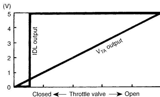
Fig. 5.16 Indication of throttle sensor voltages (Toyota)
