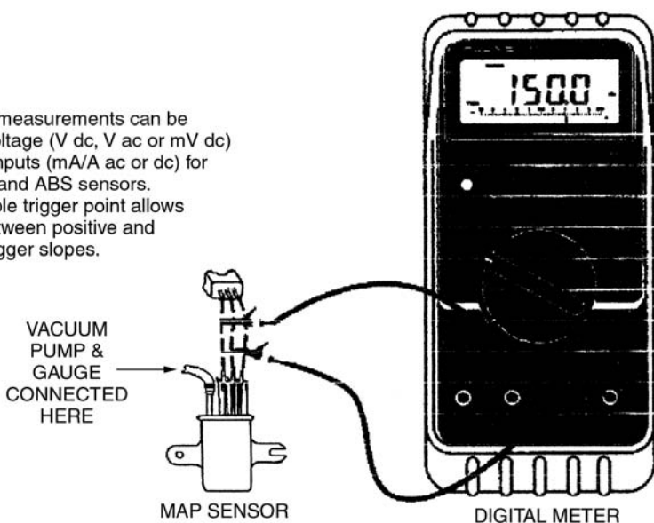
Fig. 4.19 A manifold absolute pressure sensor test
