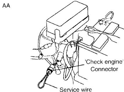
Fig. 3.4 Making the diagnostic output connection
